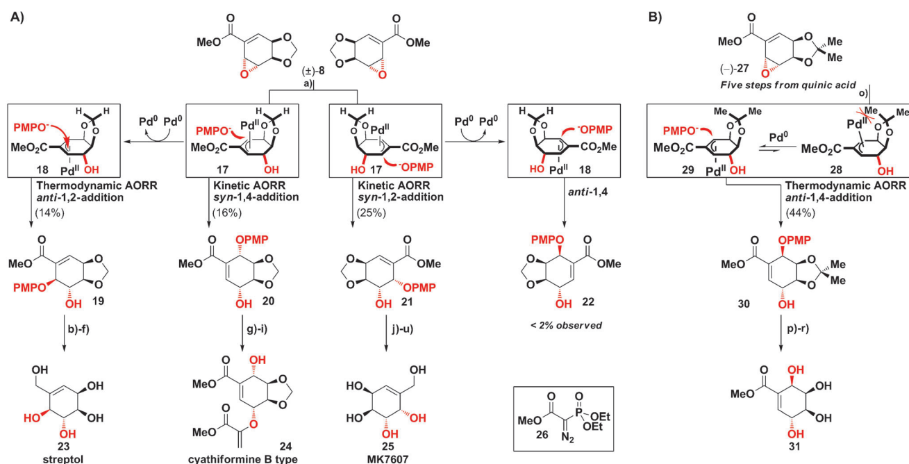
Scheme 3. Applying the AORR approach for the total synthesis of streptol, cyathiformine B type, MK7607, and a new cyclitol. A) Results with a racemic oxide; B) results when using the chiral pool. a) [\text{Pd}_2(\text{dba})_3] (10 mol %), ( R,R )- 5 (30 mol %), p - \text{MeOC}_6\text{H}_4\text{OH} (1.2 equiv), PhMe, 23 °C, 48 h (14% 19 (e.r. 90:10), 16% 20 (e.r. 90:10), 25% 21 (e.r. 92:8); b) DIBALH (3.5 equiv), \text{CH}_2\text{Cl}_2 , 0.3 h, 38%; c) \text{Ac}_2\text{O} (3.0 equiv), DIPEA, DMAP, \text{CH}_2\text{Cl}_2 , 0.3 h; d) CAN (2.2 equiv), MeCN/ \text{H}_2\text{O} 4:1, 0.20 h, 49% (two steps); e) 1) \text{AcCl} , then \text{ZnCl}_2 (0.1 equiv), 0 to 23 °C; 2) \text{H}_2\text{O} , THF, 0.3 h; f) NaOMe (1 equiv), MeOH, 16 h, 55% (two steps); g) [\text{Rh}_2(\text{OAc})_4] , 26 , \text{CH}_2\text{Cl}_2 , 5 h, reflux, 64%; h) CAN (2.2 equiv), MeCN/ \text{H}_2\text{O} 4:1, 0.20 h, 81%; i) LiHMDS, \text{CH}_2\text{O} , THF, 2 h, –78 °C, 71%; j) DIBALH (3.5 equiv), \text{CH}_2\text{Cl}_2 , 0.3 h, 28%; k) \text{Ac}_2\text{O} (3 equiv), DIPEA, DMAP, \text{CH}_2\text{Cl}_2 , 0.3 h; l) CAN (2.2 equiv), MeCN/ \text{H}_2\text{O} 4:1, 0.20 h, 21% (two steps); m) 1) \text{AcCl} , then \text{ZnCl}_2 (0.1 equiv), 0 to 23 °C; 2) \text{H}_2\text{O} , THF, 0.3 h; n) NaOMe (1 equiv), MeOH, 16 h, 57% (two steps); o) [\text{Pd}_2(\text{dba})_3] (10 mol %), ( S,S )- 5 (30 mol %), p - \text{MeOC}_6\text{H}_4\text{OH} (1.2 equiv), PhMe, 23 °C, 48 h, 44%; p) 1) \text{Ac}_2\text{O} (3 equiv), DIPEA, DMAP, \text{CH}_2\text{Cl}_2 , 0.3 h; 2) CAN (2.2 equiv), MeCN/ \text{H}_2\text{O} 4:1, 0.20 h, 63%; q) 1) NaOMe, MeOH, 0.1 h, 23 °C, 98%; 2) TFA, MeOH, 40 °C, 7 h, 51%. dba = dibenzylideneacetone, DIBALH = diisobutylaluminum hydride, DIPEA = diisopropylethylamine, DMAP = 4-(dimethylamino)pyridine, CAN = ceric ammonium nitrate, LiHMDS = lithium hexamethyldisilazide, TFA = trifluoroacetic acid.
